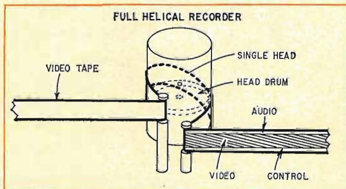
Fig. 2—Standard industrial video recorder has helical scan.
