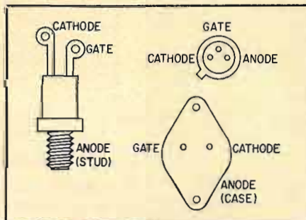
Fig. 4—Three thyristor-terminal layouts.
