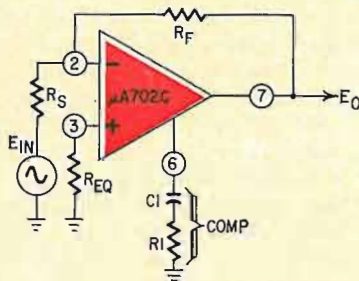
Fig. 3—How to design desired frequency response into the IC audio preamplifier.
