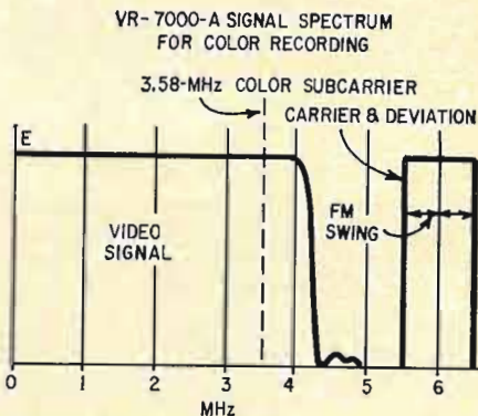
Fig. 7—The color recording bandwidth.
