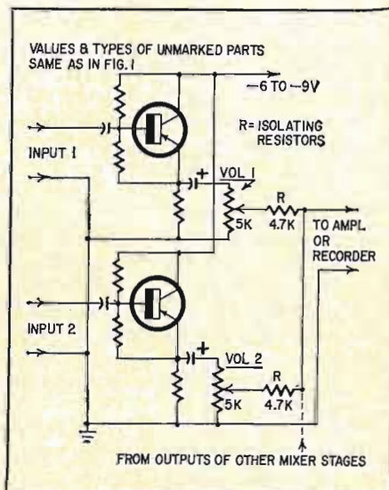
Fig. 2—Using the basic emitter followers in a simple passive resistance mixer. See text for explanation of circuits operation.
