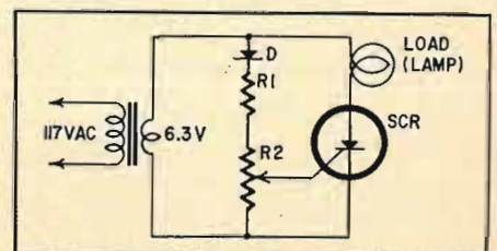
Fig. 1—Basic idea behind the checker: a simplified lamp-dimmer circuit. R1 is necessary to limit forward gate current.
