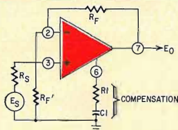
Fig. 3—How to design desired frequency response into the IC audio preamplifier.
