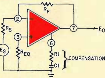
Fig. 5—With this connection, noninverting circuit of Fig. 4 becomes inverting.
