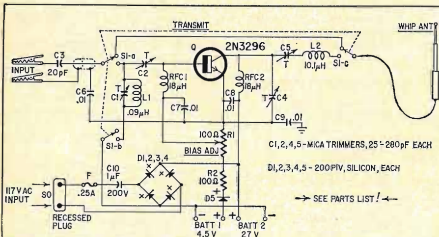
Fig. 1—Complete schematic of the linear amplifier. Ac plug is TV chassis type.
