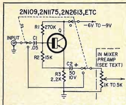
Fig. 1—Circuit of an emitter follower the author used to step up input impedance of a mixer described in R-E for March 1963.
