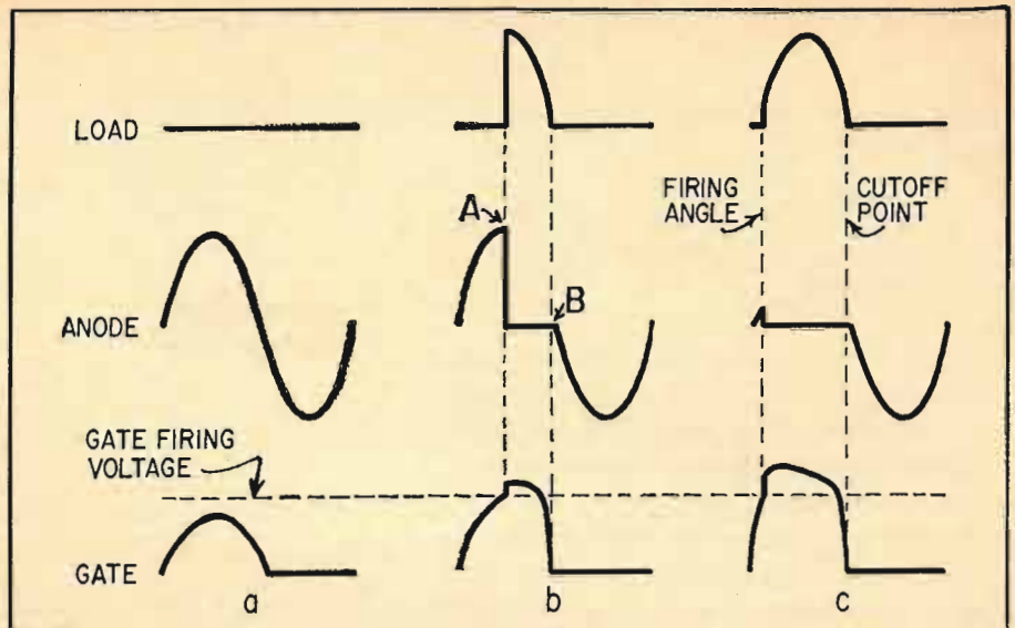
Fig. 2—These waveforms show what occurs inside the checker for three settings of R2.
