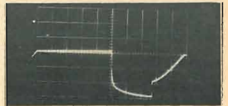
Fig. 6—Waveform across the SCR (a) and at gate (b) at minimum firing angle.
