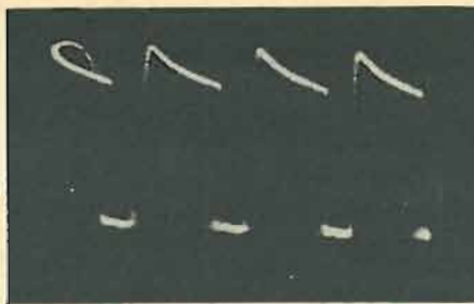
Fig. 1—Typical voltage waveform at collector of horizontal-output transistor.
